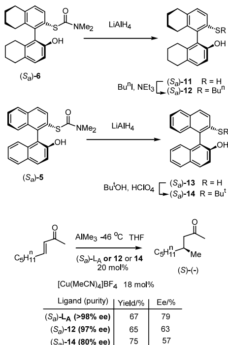
Scheme 4. Ligand preparation and testing in asymmetric catalytic conjugate addition of \text{AlMe}_3 to nonenone.
