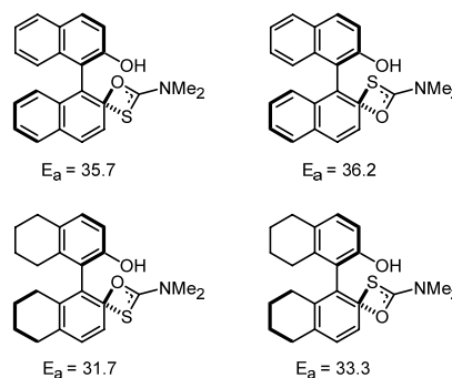
Figure 3. PM3 calculated activation energies (kcal mol -1 ) for rearrangements 3 to 5 and 4 to 6 .
