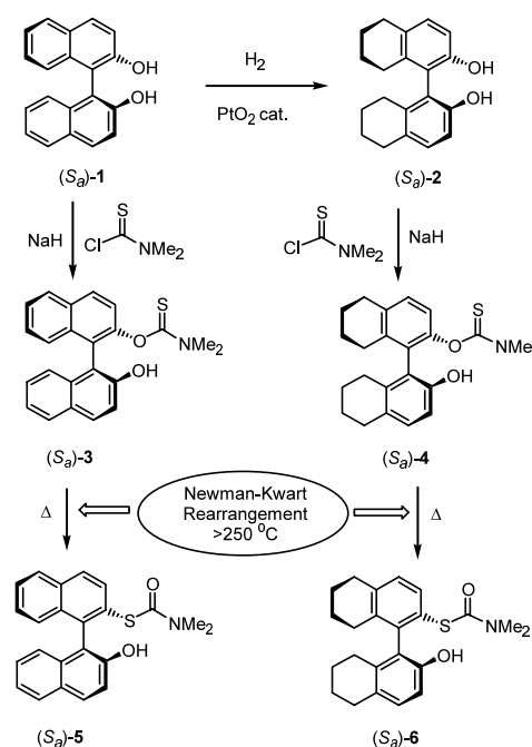
Scheme 1. Preparation of thiocarbamates from BINOL and \text{H}_8 -BINOL and their rearrangement.
