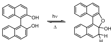
Scheme 2. Known isomerisation of BINOL.
