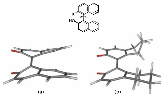
Figure 1. Lowest energy ( syn -) transition state structures found for (a) binaphthyl and (b) octahydrobinaphthyl systems (2,2'-substituents omitted for clarity).
